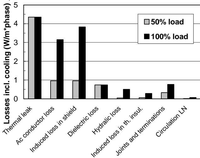
Fig. 2. Distribution of losses on primary components in a 450 MVA 132 kV HTS cable system with room temperature dielectric design at 50% and 100% load. The efficiency of the cooling machine is included in the loss components. At full load there is three major contribution to the loss, and at half load only one major loss component exist namely the thermal leak loss.
