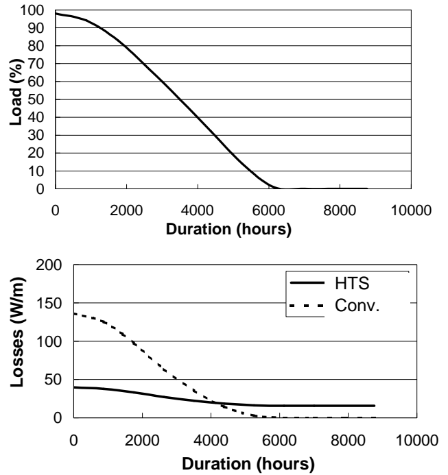
Fig. 6. Load profile and loss in HTS and conventional cable system for a connection between a offshore windmill park and the network. Data covers a year (8760 hours).
