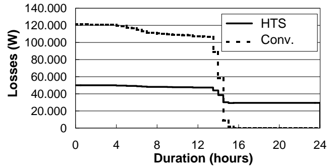
Fig. 4. Load profile and loss in HTS and conventional cable system for a 2.5 km connection between a combined heat-power plant and the network. The data covers a representative 24 hour period.
